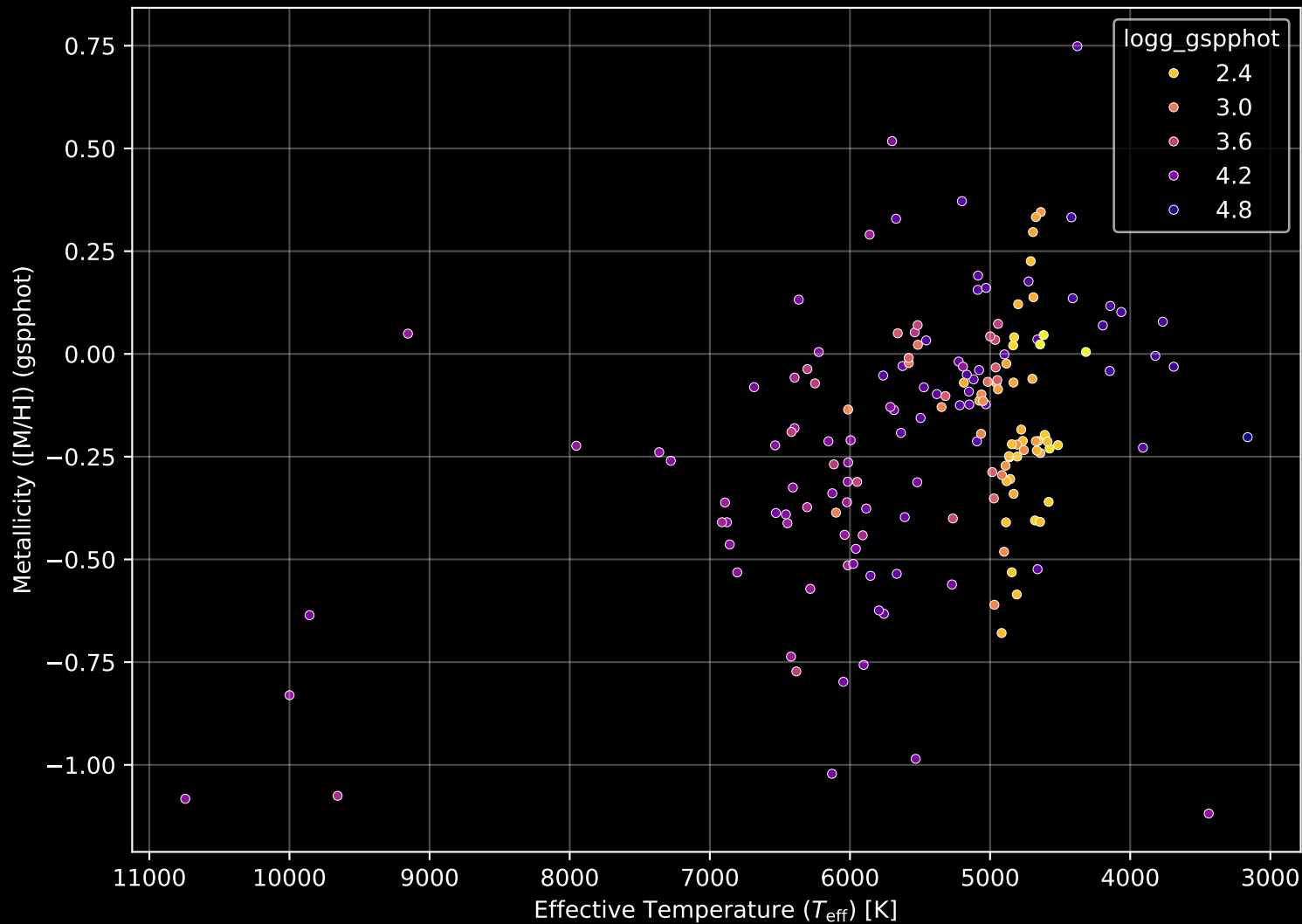
APOGEE DR17 Field: [CVZTILE_104+30_btx] Stellar Population Parameters (n= 169)
