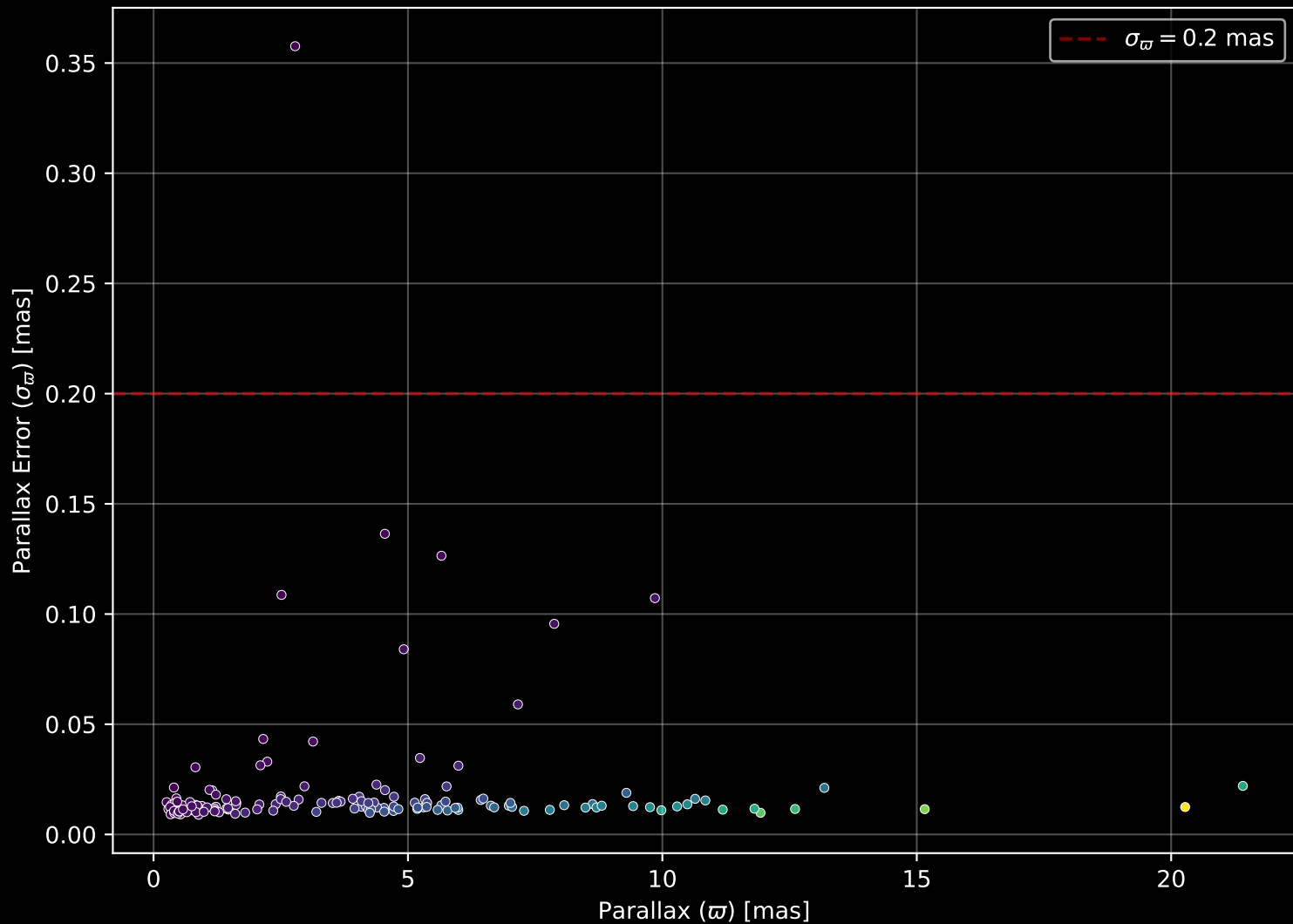
APOGEE DR17 Field: [CVZTILE_104+30_btx] Parallax Quality (n= 169)
