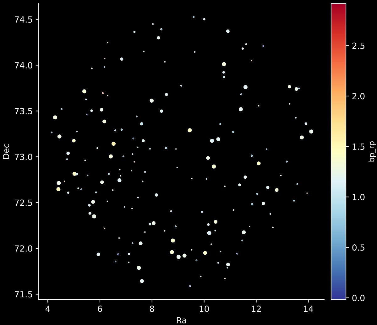
APOGEE DR17 Field: [CVZTILE_104+30_btx] Stars: 169
