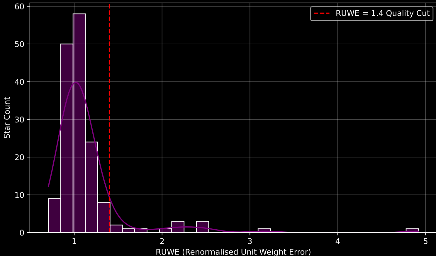
GAPOGEE DR17 Field [CVZTILE_104+30_btx] RUWE Distribution (n= 162)
