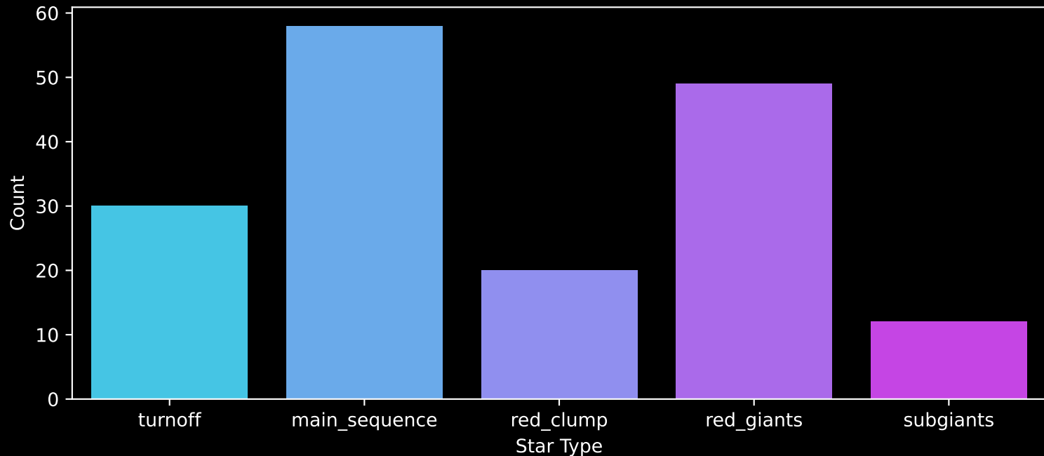
APOGEE DR17 Field: [CVZTILE_104+30_btx] Count plot of Star Type
