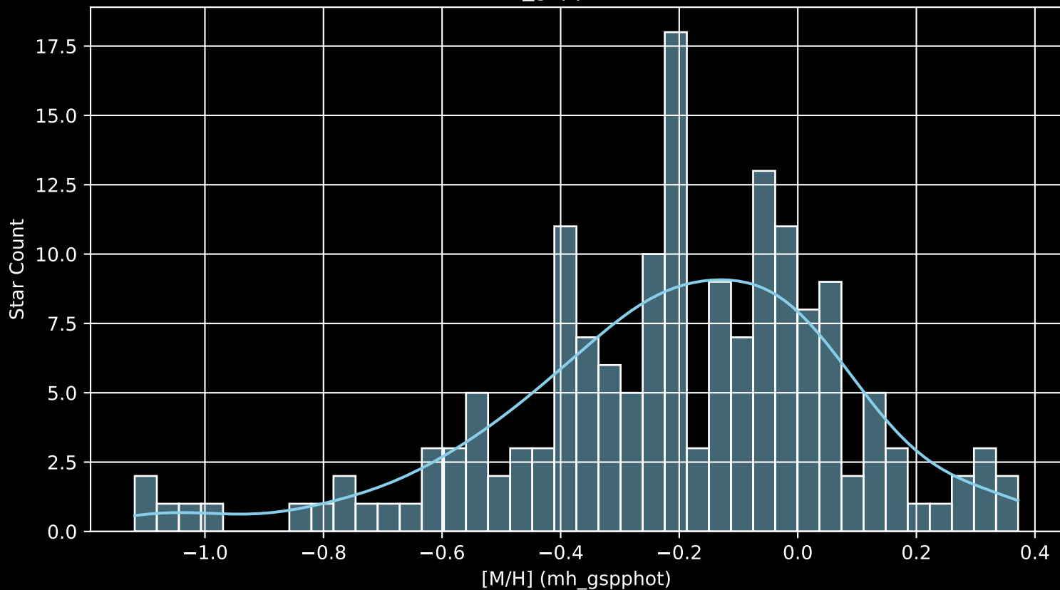
APOGEE DR17 Field: [CVZTILE_104+30_btx [M/H] (mh_gspphot) (n= 167)
