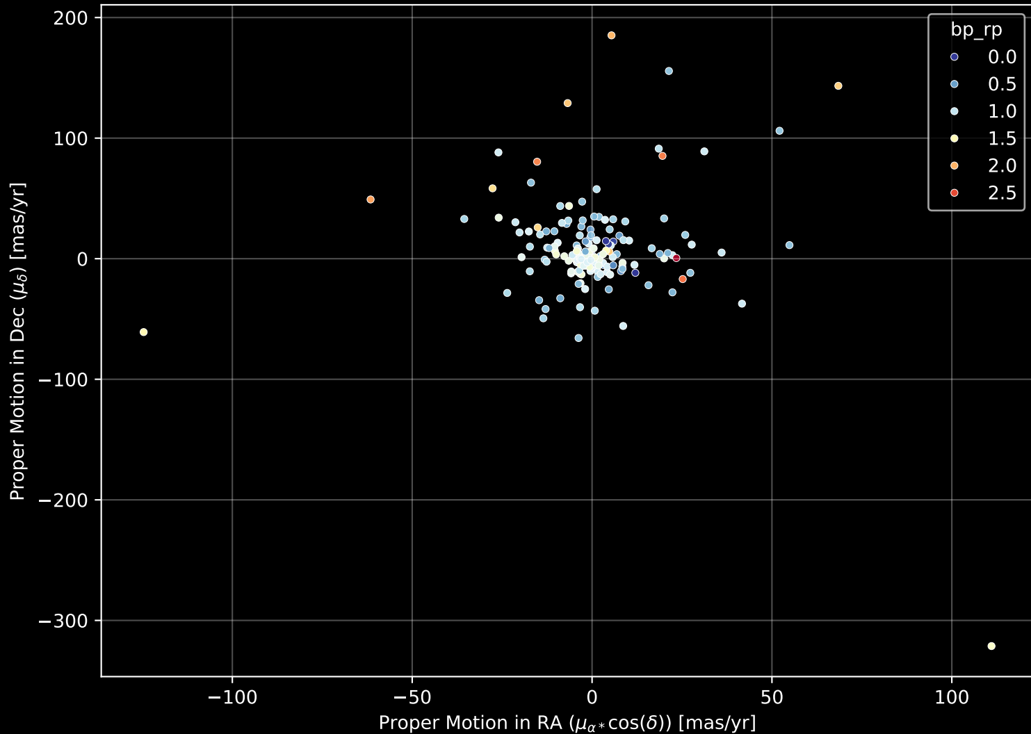
APOGEE DR17 Field: [CVZTILE_104+30_btx] Proper Motion Diagram (n= 169)
